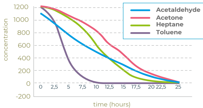
Reduction in VOCs on Clean&Fresh Treated Glass
